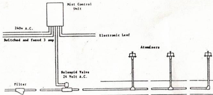
Fig.3 Installation Arrangement
